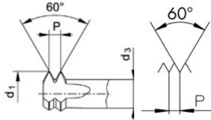
Profile sketch
