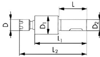
Technical drawing
