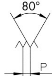
Profile sketch
